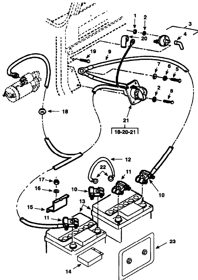
CONNECTION LEADS, MAIN SWITCH AND POWER RECEPTACLE
